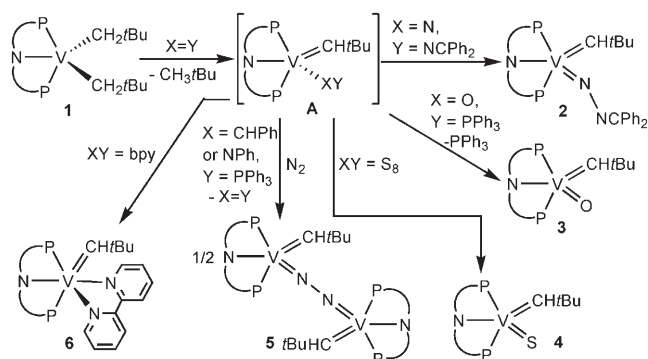
Scheme 1. Synthesis of complexes 2–6 via intermediate A and from the bis-neopentyl– V^{III} precursor 1 . The N[2-P(CHMe)_2-4-methylphenyl]_2 framework has been simplified to the PNP cartoon.
